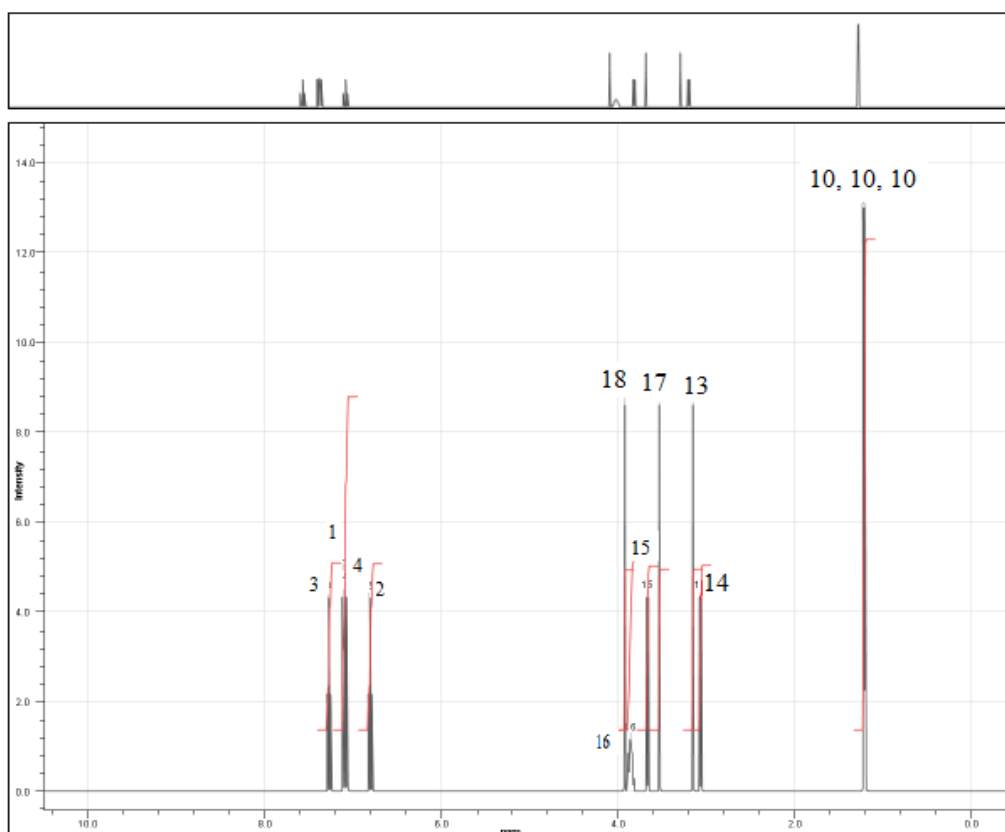
Figure 33: Better resolution of ^1\text{H} -NMR spectrum of (AZ-1) by Marvin Sketch.
